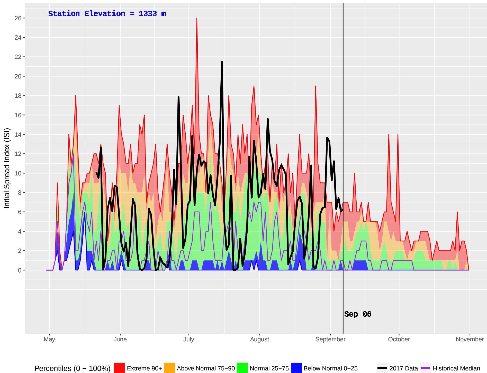
GOLDSTREAM 2 (919) : Historical (2005–2016) and Current (2017) Noon Initial Spread Index (ISI)
