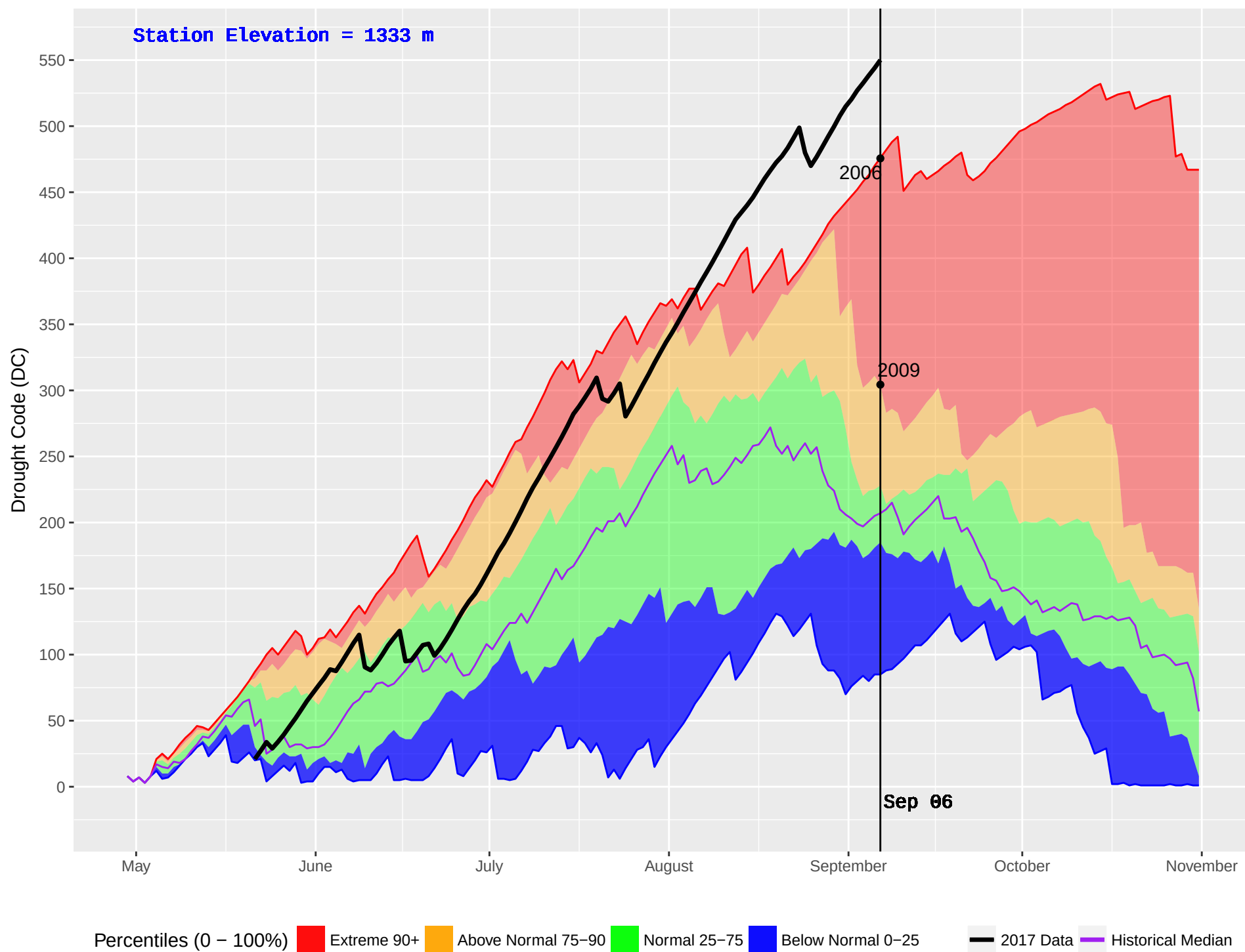
GOLDSTREAM 2 (919) : Historical (2005–2016) and Current (2017) Noon Drought Code (DC)
